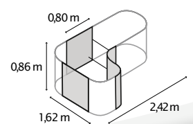
EXTENSION VITA CURVE
